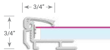
SupraSlim Profile
